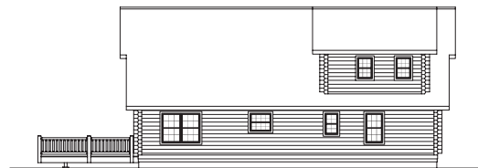
REAR ELEVATION
