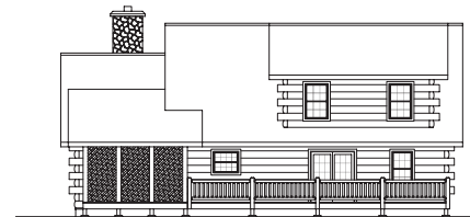
REAR ELEVATION
