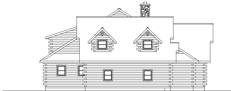
LEFT ELEVATION
